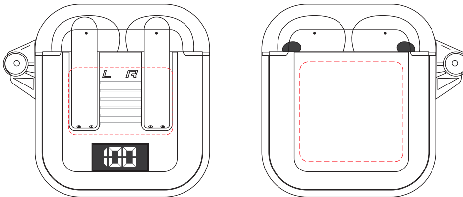
FRONT Branding Area: 28 x 18 mm 4CP Direct Digital Print / Pad Print
