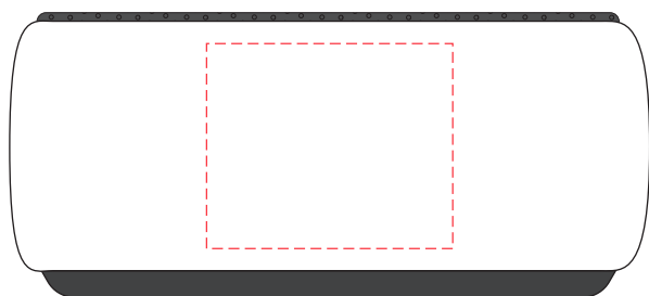
Front Side Branding : 30 x 25 mm (w x h) Pad Print
